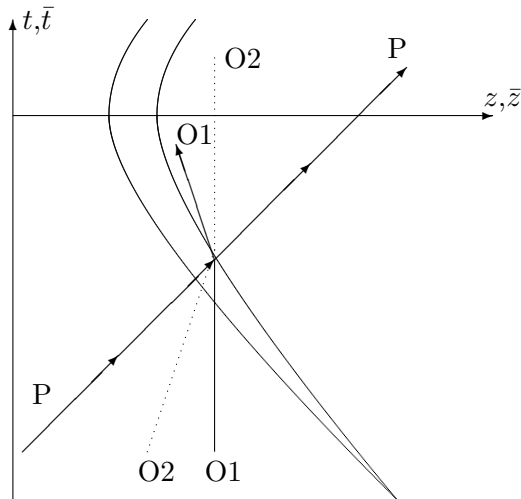
Figure 2. Close up view of the motion of bradyons and photons encountering a Case I wall. This is an illustration of the focusing effect of such walls. The boundaries of the wall are represented by the two curved lines. The labels correspond to the different paths: P=Photon, O1=Observer 1 (initially at rest), O2=Observer 2 (emerges at rest).
