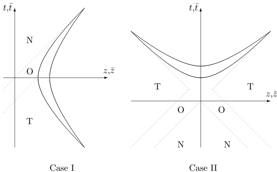
Figure 4. Illustration of the different photon-wall interactions. The regions are separated by dotted lines. The regions of space-time labeled T show the regions from which photons headed toward the wall will enter the wall transversely and lose intrinsic energy. Photons originating in the regions labeled O will enter the wall obliquely and gain intrinsic energy. The regions labeled N mark those regions from which photons are prohibited from interacting with the wall.
