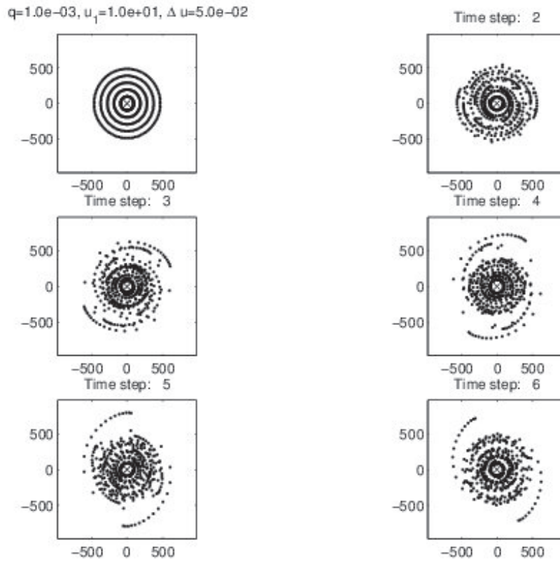
Figure 6. Simulation results of the interaction of a case II wall with a toy galaxy. The units on the axis are in hundreds of parsecs. The wall parameters ( q , u_1 and \mu ) are given above the initially circular distribution. The time interval between the plots is about one-tenth the time it would take this initial distribution to complete one complete rotation.
