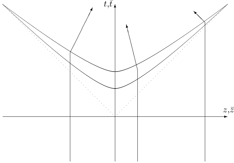
Figure 3. Illustration of the focusing effect csae II walls have on different bradyons which were initially at rest in region 1. Notice that the wall has a greater effect on bradyons further from z = 0 .
