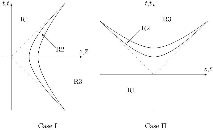
Figure 1. Schematic of the two cases of tachyon walls. In both cases the wall is infinite in the x and y directions, which have been suppressed in the illustration. The dotted lines mark the limiting boundaries of the wall. R1 and R3 mark regions 1 and 3 (outside the wall), while region 2 marks the wall interior.
