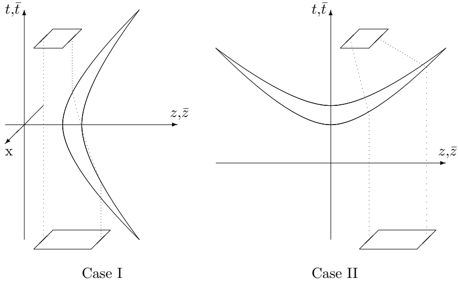
Figure 5. Extended objects which have been compressed (in the z direction) after an interaction with each case of tachyon wall. The x direction is shown in these diagrams to emphasize that only the z -width of the object is affected by the wall.
